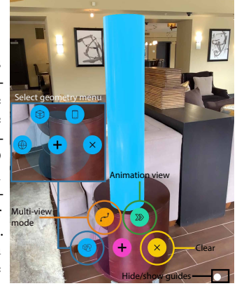
Figure 6: The user interface of our tool. Users can choose to create a curve in multi-view mode; view animations on their curves using the animation view; clear all transient geometries and curves in the environment; and also hide or show the geometry guides (i.e. mesh or transient geometry).
