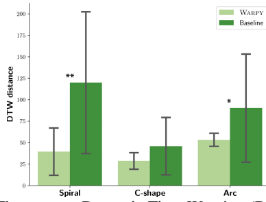
Figure 11: The average Dynamic Time Warping (DTW) distance between the created curves and the ground truth curves. A lower DTW distance means a curve is more similar in shape to the ground truth curve. The error bars represent the standard deviation.
